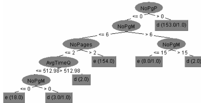
Fig. 2. Decision Tree graph for Dataset 3
