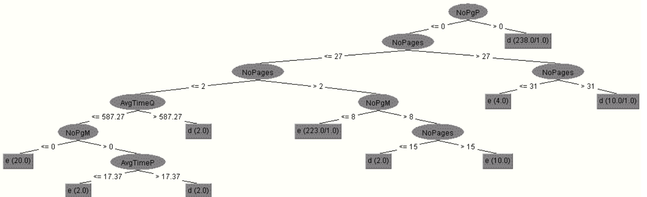
Fig. 3. Decision Tree for dataset DS4_S2
